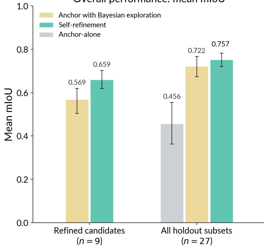
Overall performance: mean mIoU
