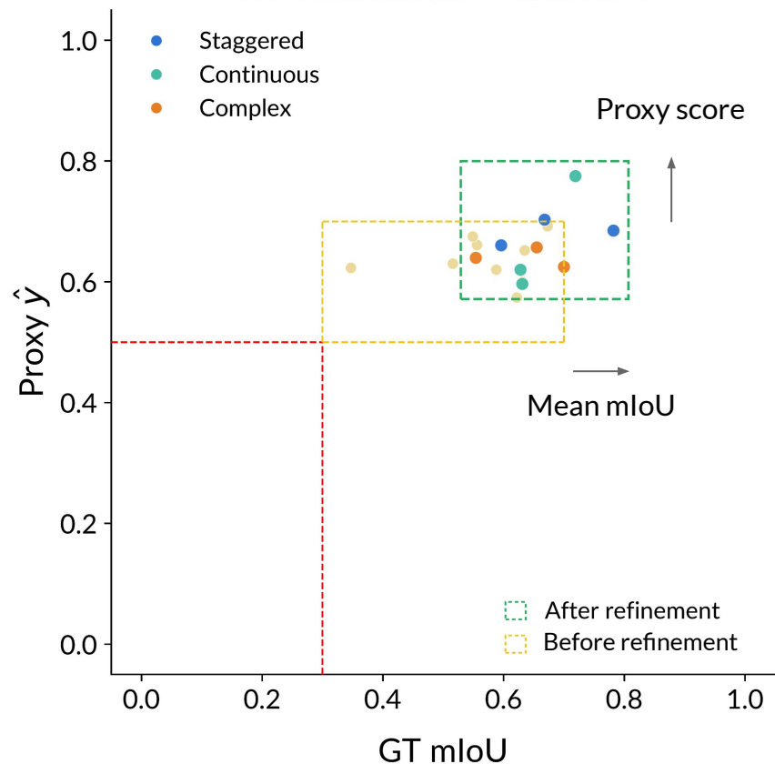
Self-refinement: 9 candidates
