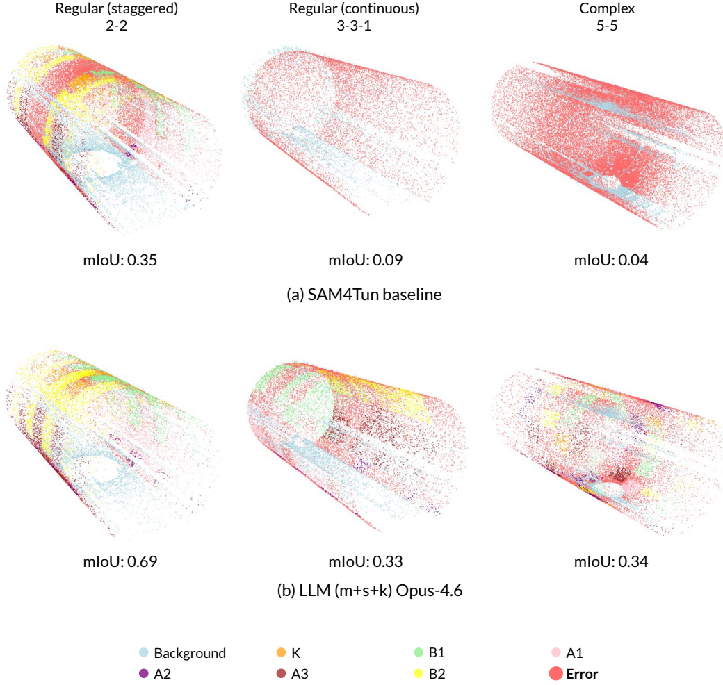
Figure 9: Point-cloud visualisation for the tunnels with the largest mIoU gain in each category: regular (staggered; 2-2), regular (continuous; 3-3-1), and complex (5-5). Top (a): SAM4Tun baseline; bottom (b): LLM-adapted pipeline (m+s+k, Opus-4.6). Colours indicate classes; red denotes error; mIoU is shown per example.
