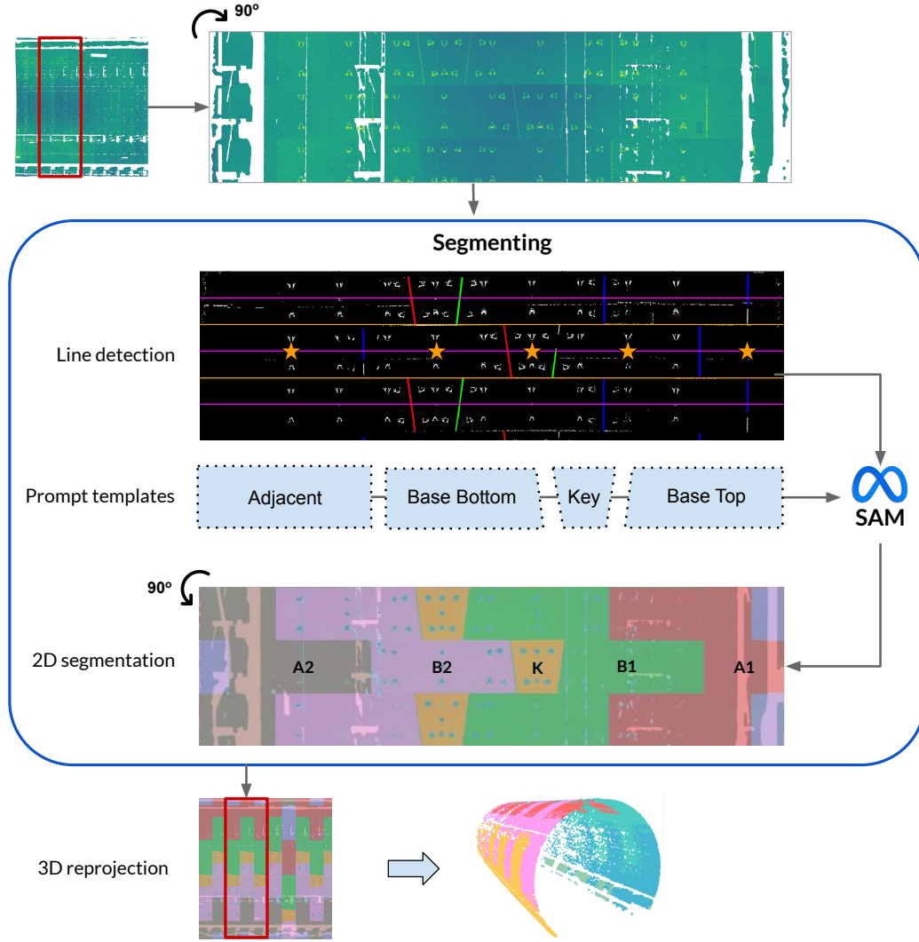
Figure 5: Stage 4-Segmenting: Hough-transform line detection [42] to identify ring boundaries, constructs template-based prompts, and feeds them to SAM [11], which produces 2D segment masks that are reprojected into 3D. (Note: rotation is shown for visualisation purposes only.)
