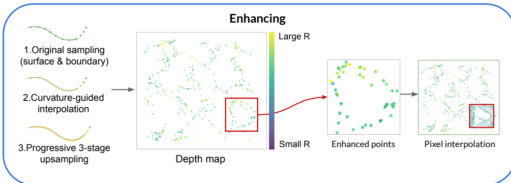
Figure 4: Stage 3-Enhancing. Left: curvature-guided surface and boundary interpolation along the tunnel lining, showing original sampling, curvature-guided insertion, and progressive three-stage upsampling. Centre: unfolded 2D depth map after enhancement, where inserted points improve geometric continuity; the red box highlights a local region of interest. Right: zoomed views of the highlighted region, showing added points and pixel-level interpolation.
