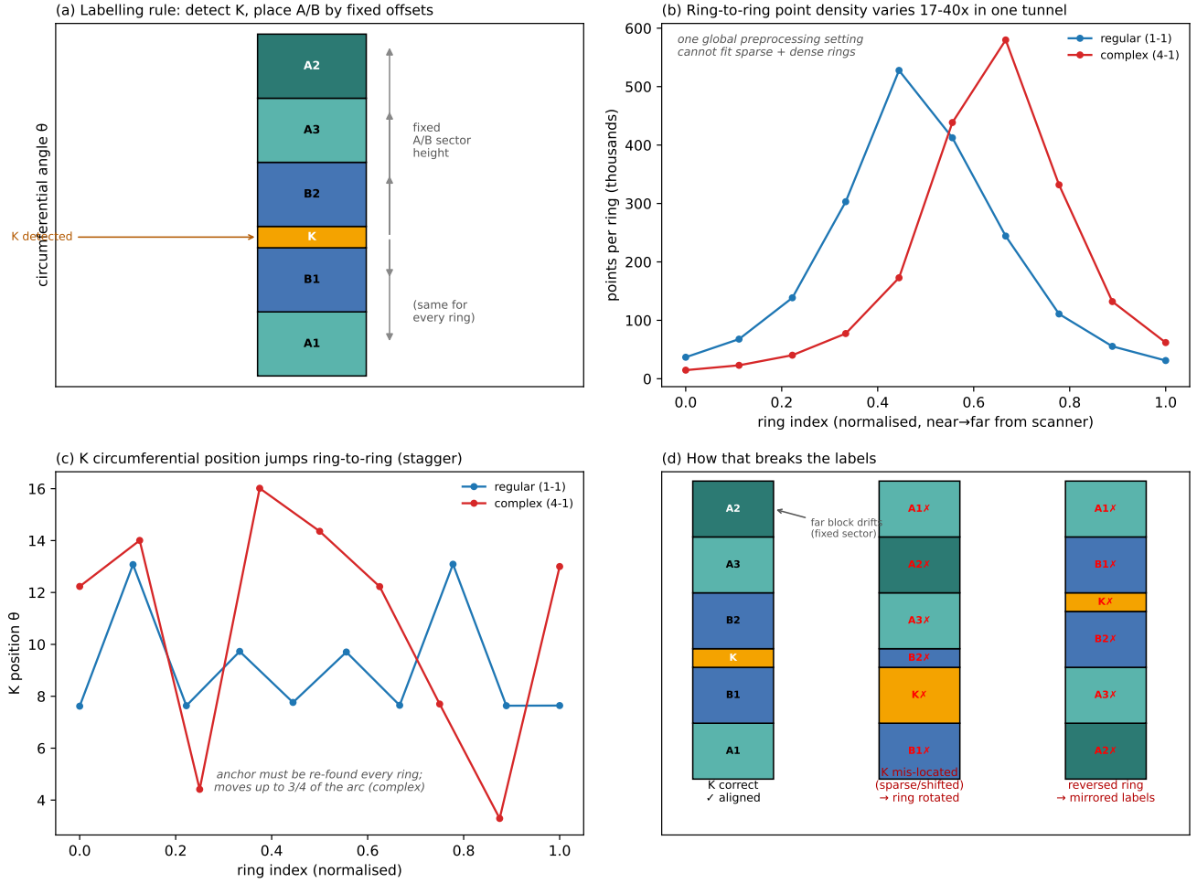
Figure 12: Why class confusion arises. (a) Blocks are labelled by position: detect the key block K, then place all other blocks by a fixed angular offset shared across rings and tunnels. (b) Within one tunnel, ring point density varies by 17–40 \times in a single-peaked scanner profile, so no single preprocessing setting fits both the densest and sparsest rings. (c) The K anchor is not fixed: staggered assembly shifts its circumferential position from ring to ring, by up to a third of the arc on a regular tunnel and three quarters on a complex one. (d) Resulting failures: a mis-located K rotates the whole ring’s labels, the fixed sector drifts for blocks far from K, and a reversed ring handedness mirrors the labels.
