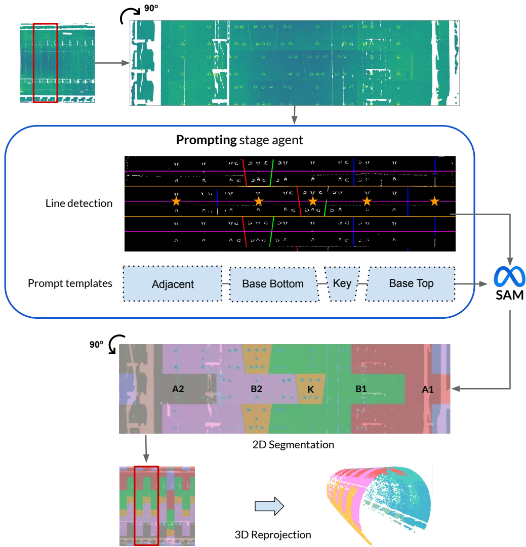
Figure 6: Stage 4—Segmenting. The segmenting stage applies Hough-transform line detection [?] to identify ring boundaries, then constructs template-based prompts and feeds them to SAM [?]. SAM produces 2D segment masks that are reprojected into 3D. (Note: rotation is shown for visualisation purposes only.)
