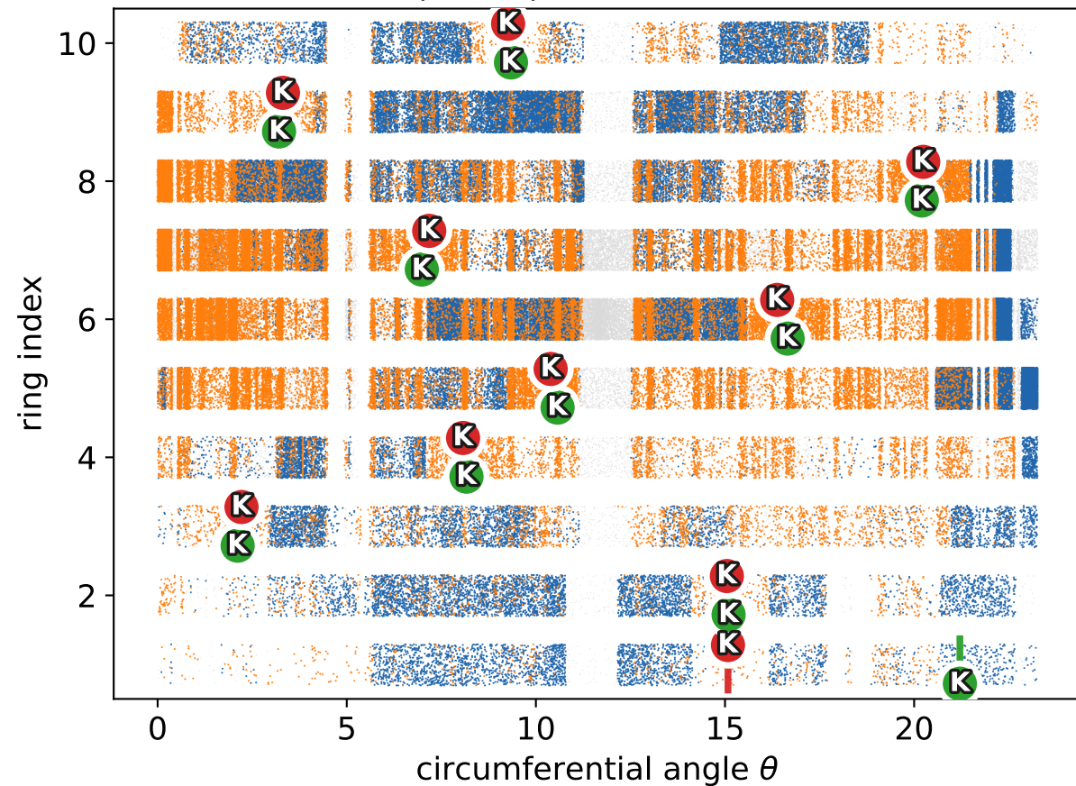
(a) Tunnel 5-5 (complex, Opus-4.6 m+s+k) — FN 11% FP 6%
