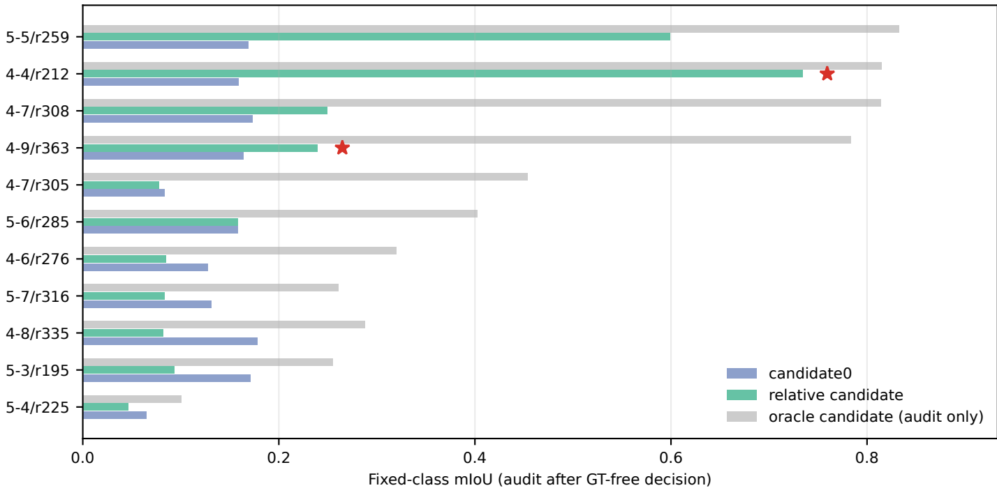
Relative proxy challenge audit: accepted stars, conservative abstention elsewhere
