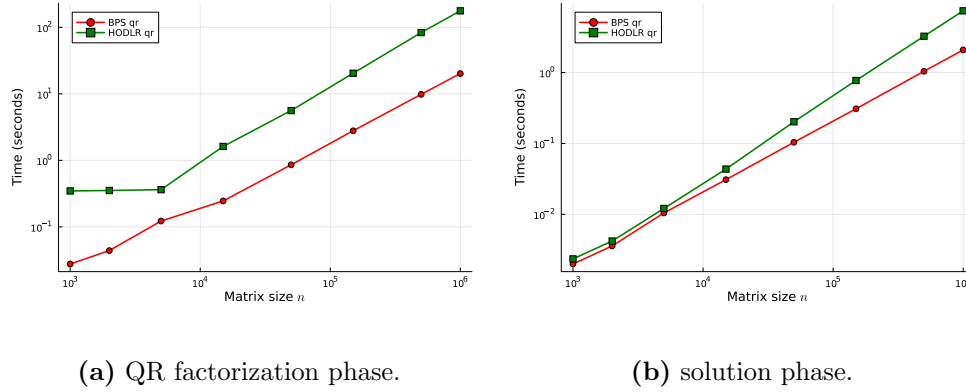
FIG. 4. Log-log performance comparisons between our proposed fast BPS QR algorithm and the HODLR QR implementation from [16] (with parameters \ell = 4 , m = 5 , r = 2 , p = 3 ). Panel (a) illustrates the execution times for the structured QR factorization phase; Panel (b) presents the execution times for the solve phase (applying Q^T and backward substitution).
