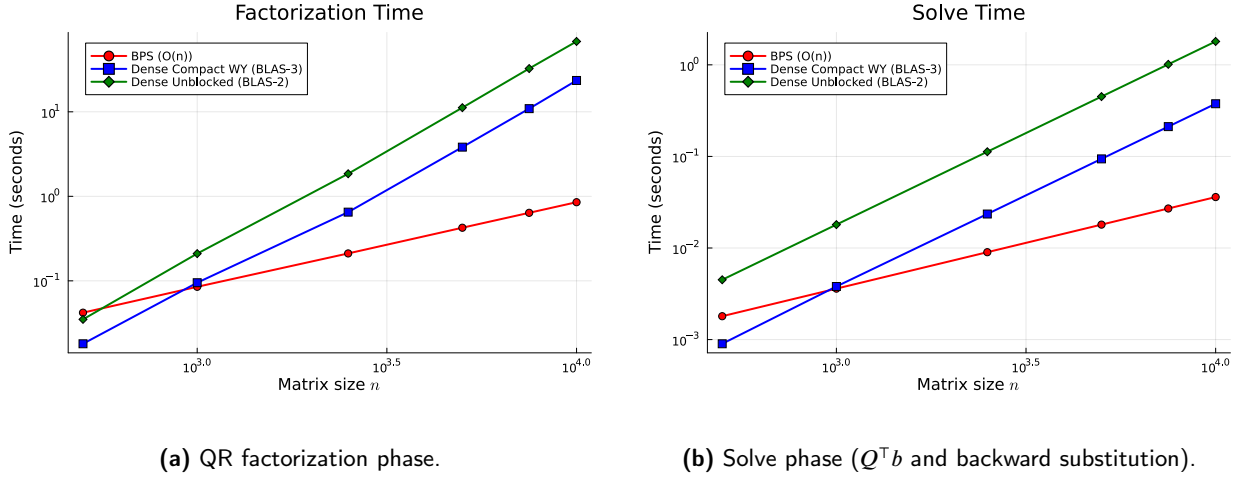
Figure 4: Performance scaling comparison between our proposed structured O(n) BPS solver and LAPACK dense solvers (both Unblocked and Compact WY BLAS-3 implementations). Panel (a) shows the execution times for the QR factorization phase; Panel (b) illustrates the execution times for the solve phase.
