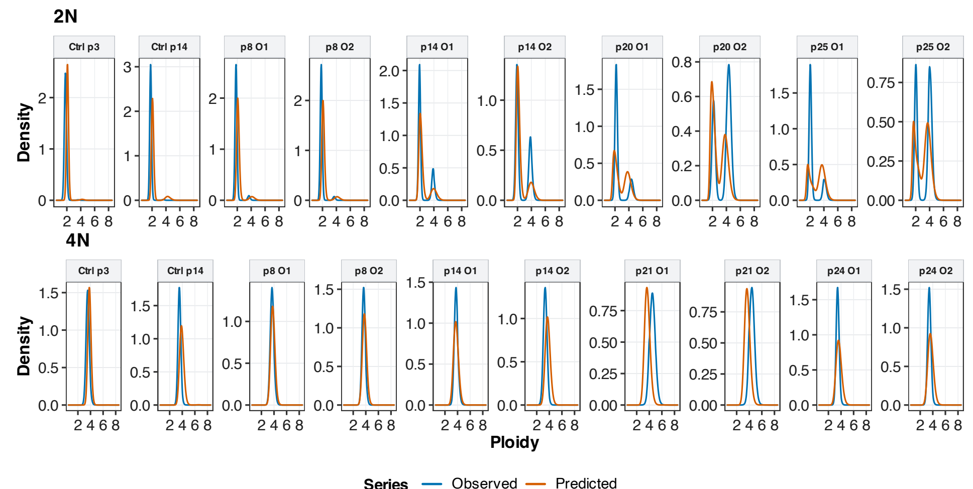
B. Observed versus predicted G0/G1 ploidy-density curves
