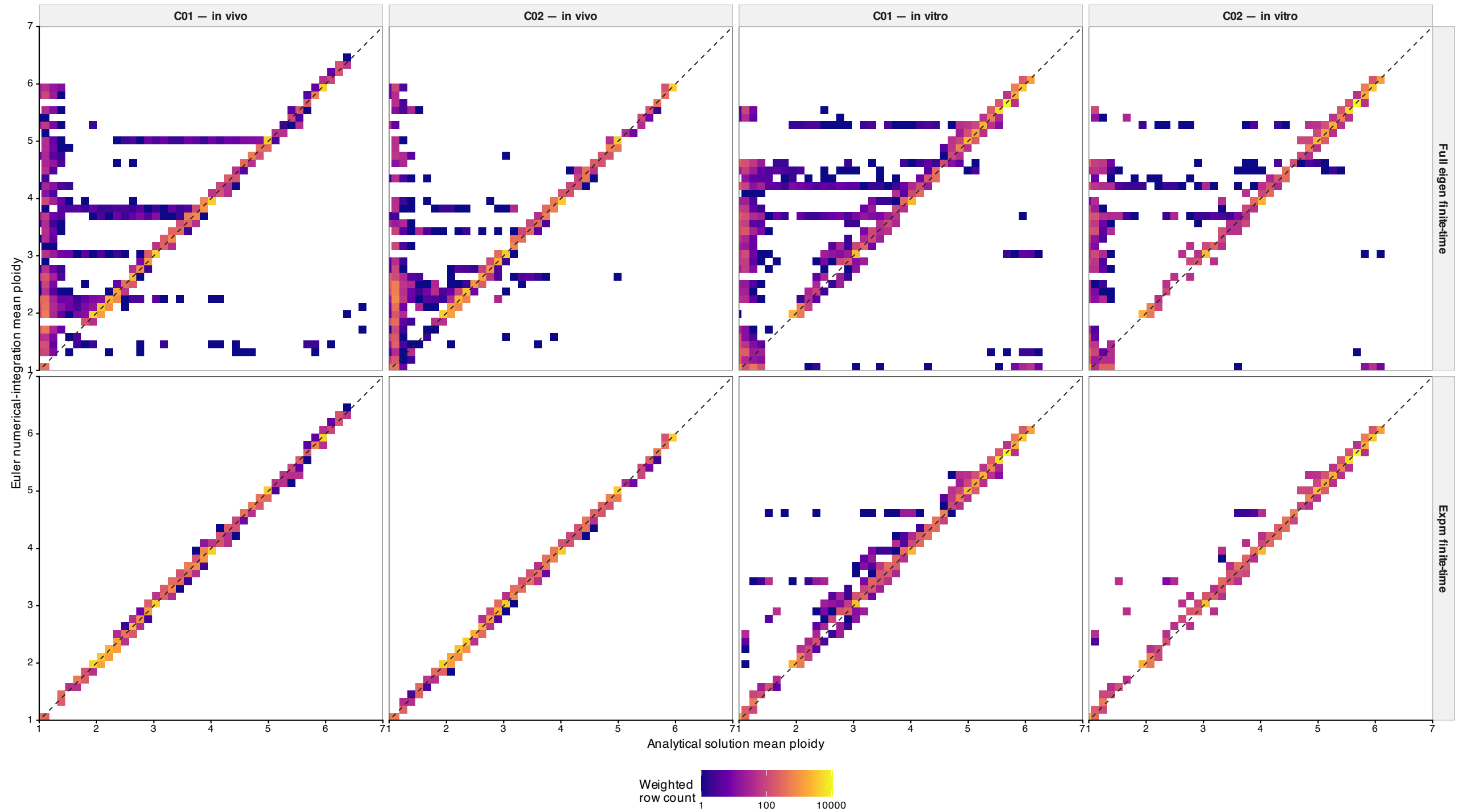
Finite-time analytical solutions versus Euler numerical integration
