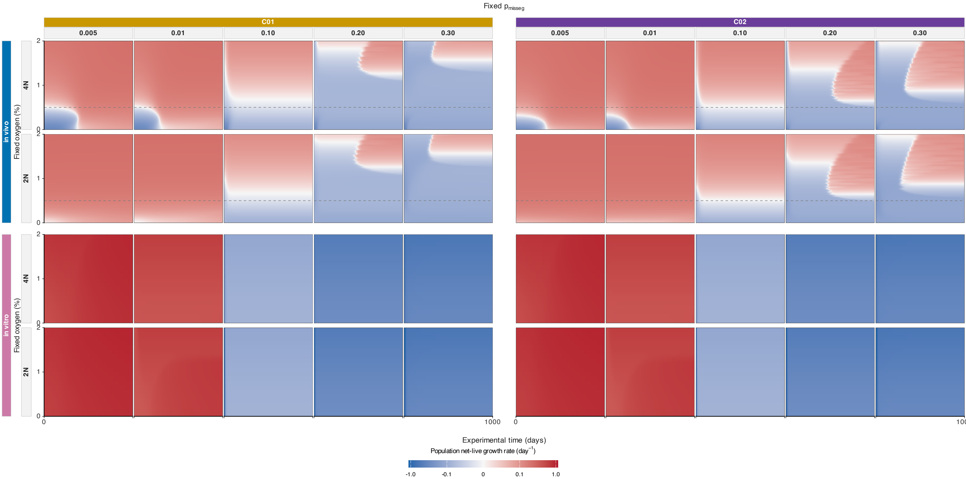
Population-weighted net-live growth rate (signed pseudo-log10 colors)
