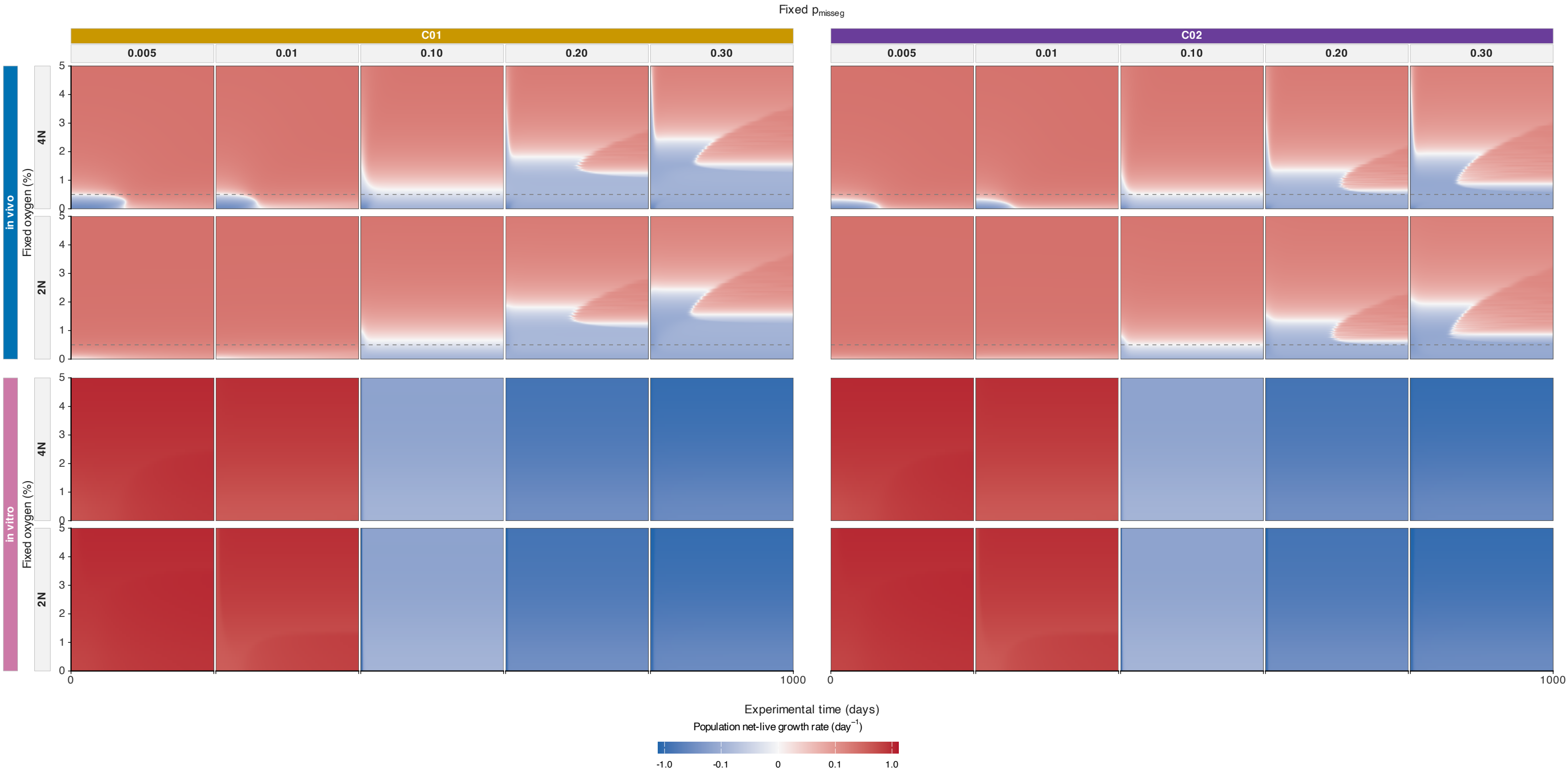
Population-weighted net-live growth rate (oxygen 0-5%; signed pseudo-log10 colors)
