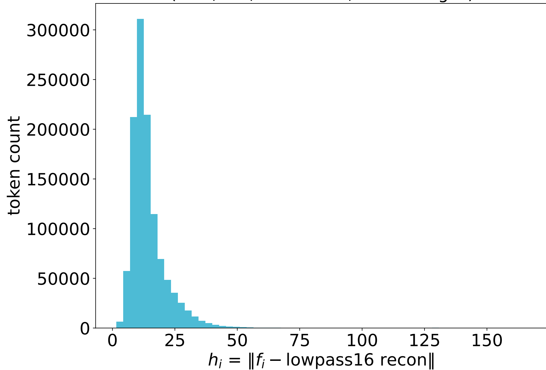
residual distribution (n=1,152,000 tokens, 2000 images)
