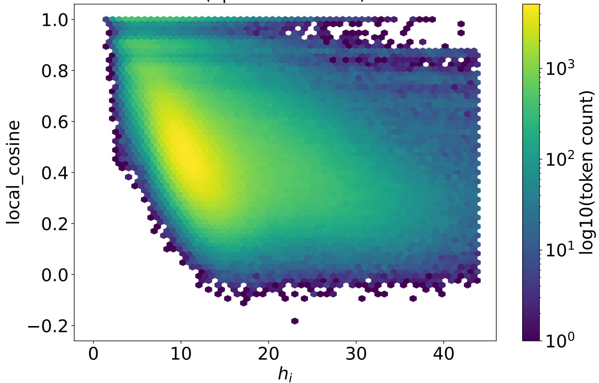
h_i vs local_cosine (Spearman=-0.49)
