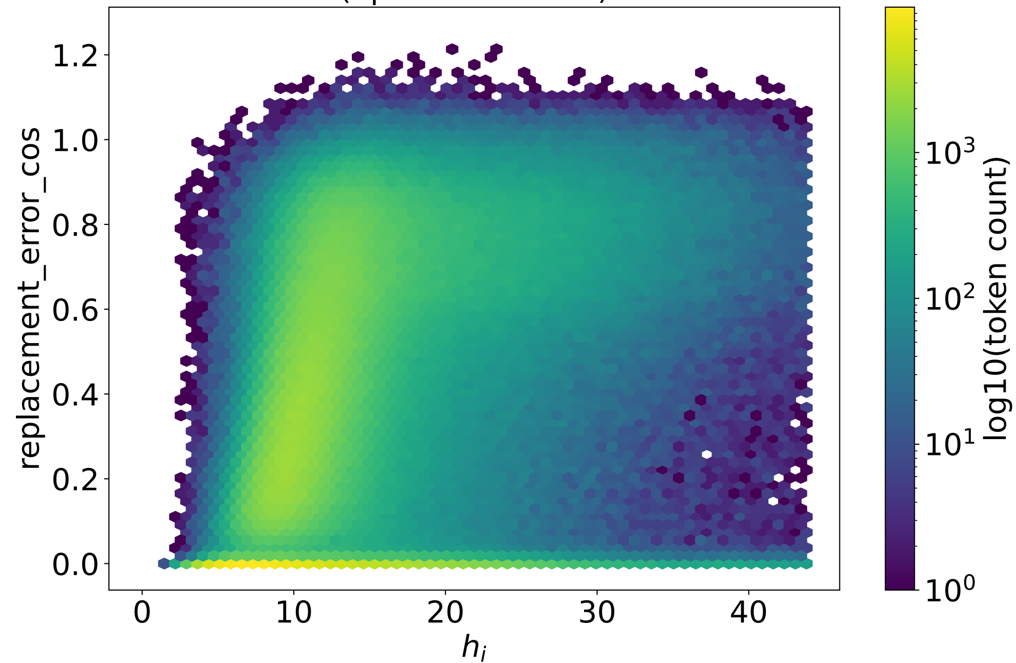
h_i vs replacement_error (Spearman=0.43)
