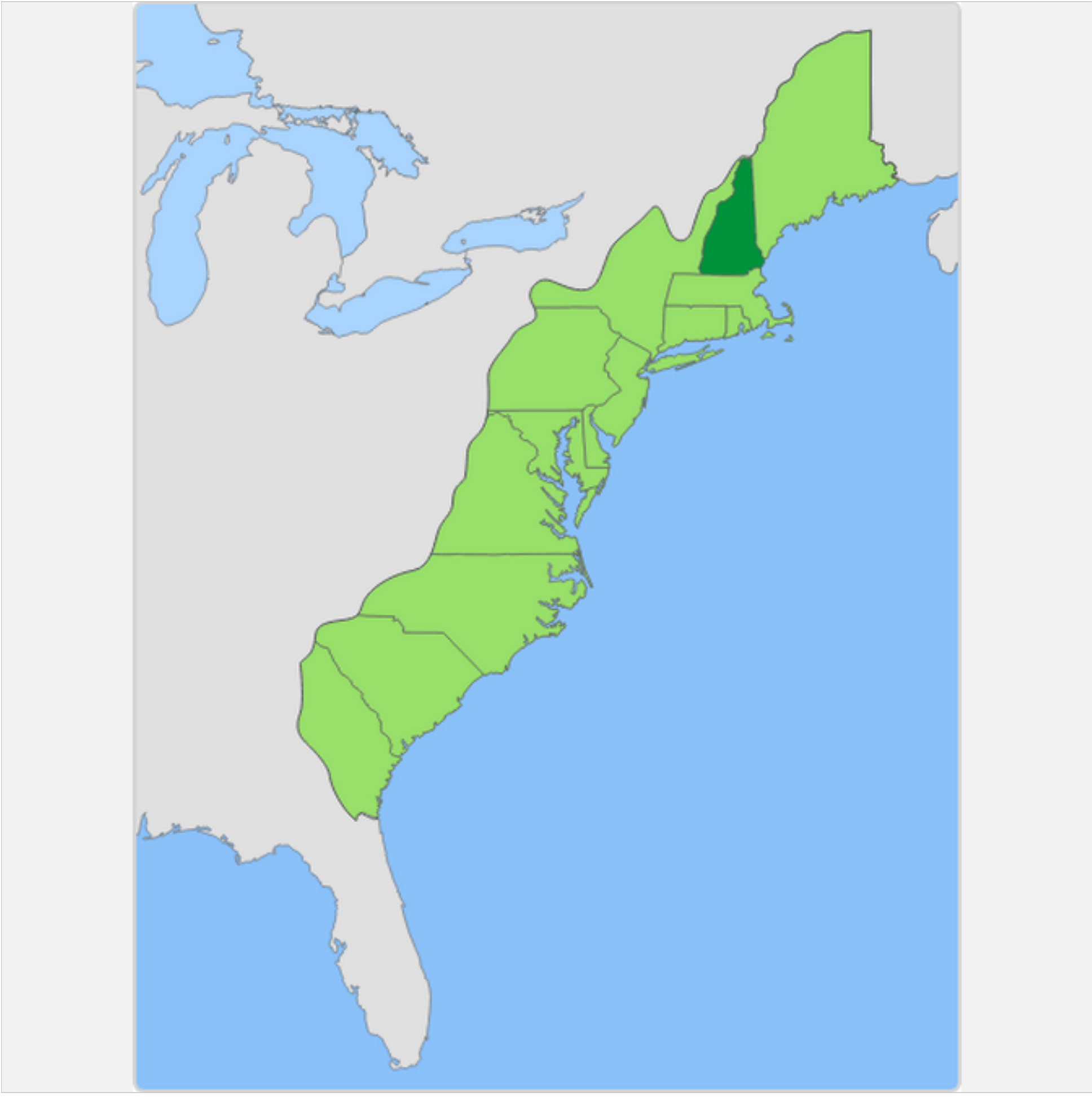
ScienceQA-IMG
