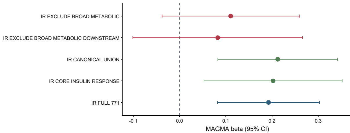
b Leave-one-pathway-out estimates
