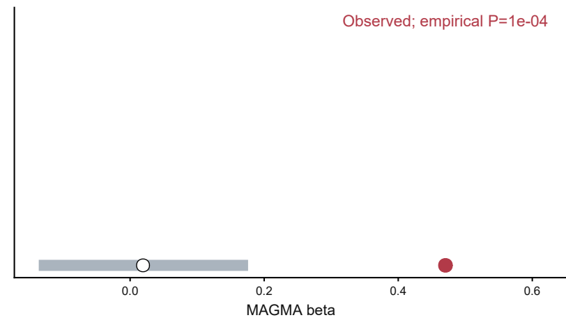
c Size-matched random gene sets
