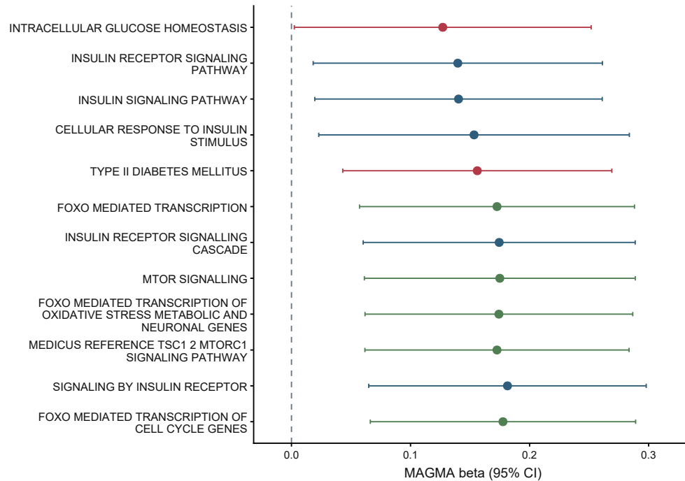
b Leave-one-pathway-out estimates
