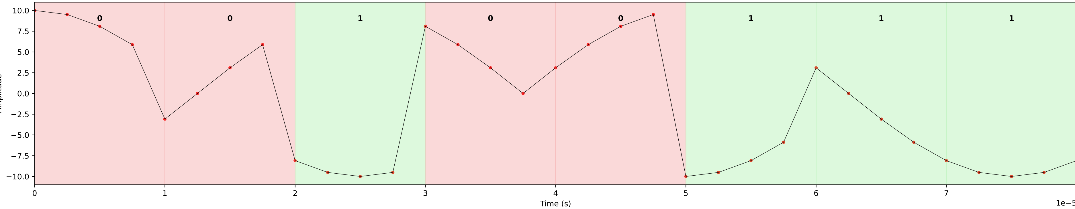
Received Signal with Detected Bit Labels
