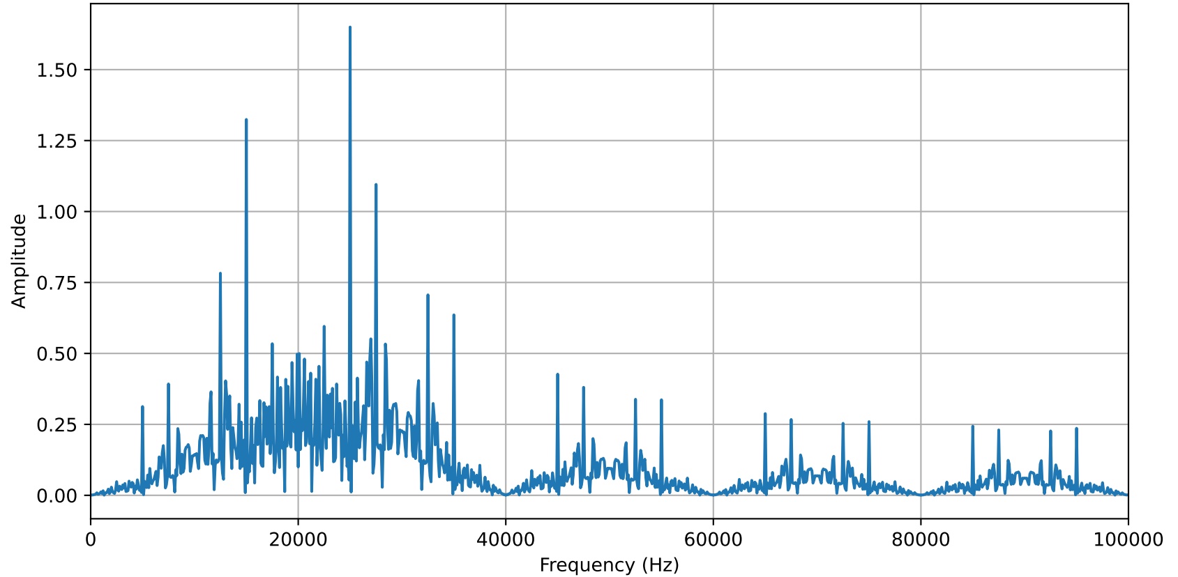
FFT of Received Signal
