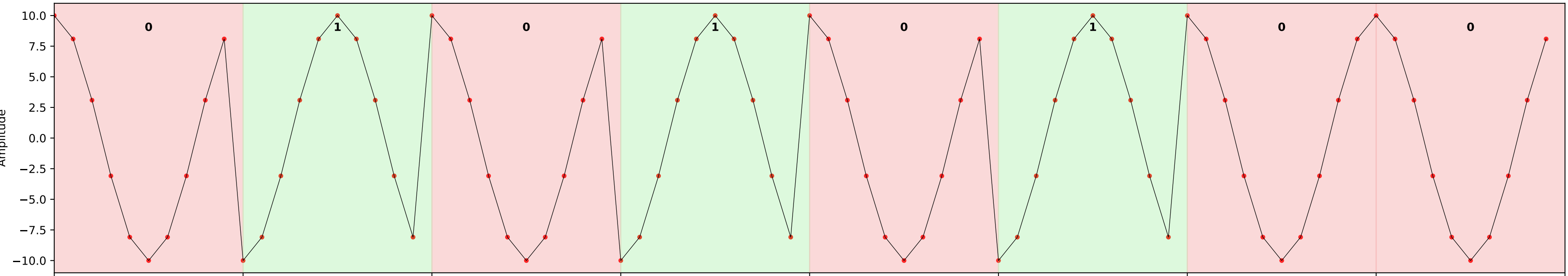
Received Signal with Detected Bit Labels
