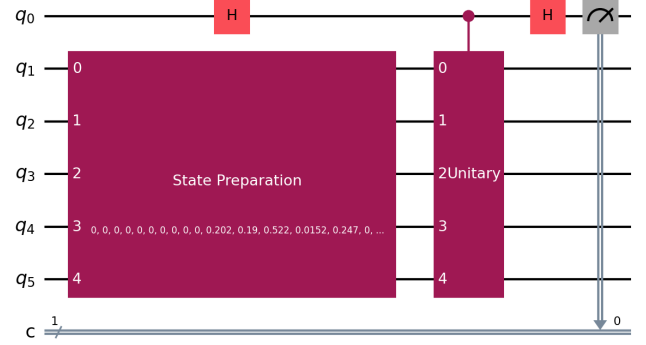
Fig. 5. Circuit diagram of the ISDO-B implementation. The controlled transition unitary U_{\chi\psi} is used to estimate the linear overlap \text{Re}\langle\phi|\psi\rangle by measuring the ancilla qubit expectation value over a small constant number of shots.
