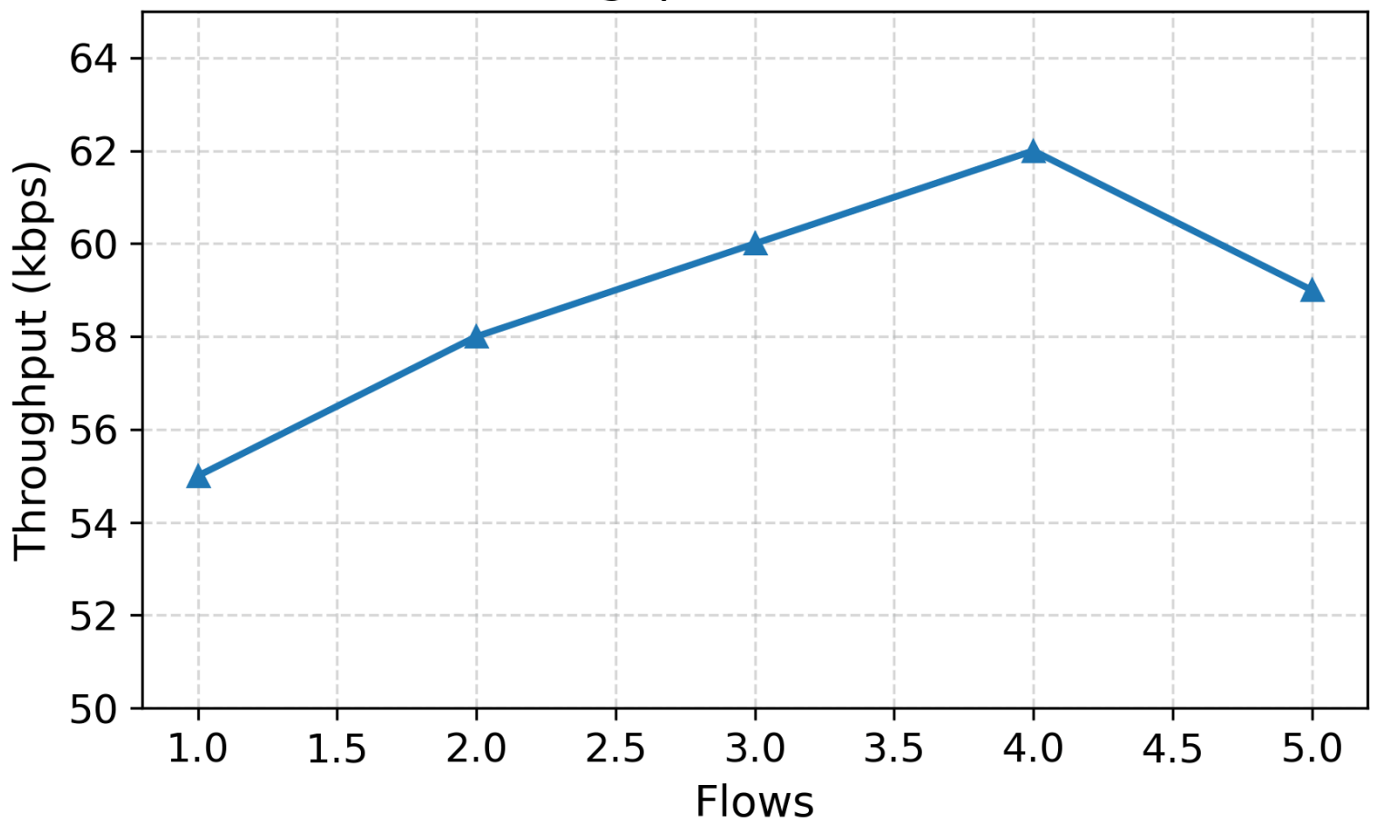
Throughput Performance
