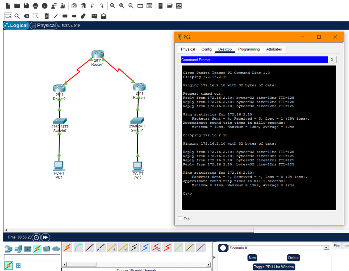
Screenshot showing network topology and successful ping from PC2 to PC1
