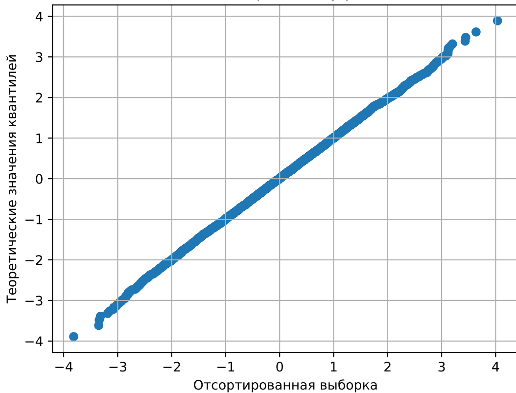
normal probability plot
