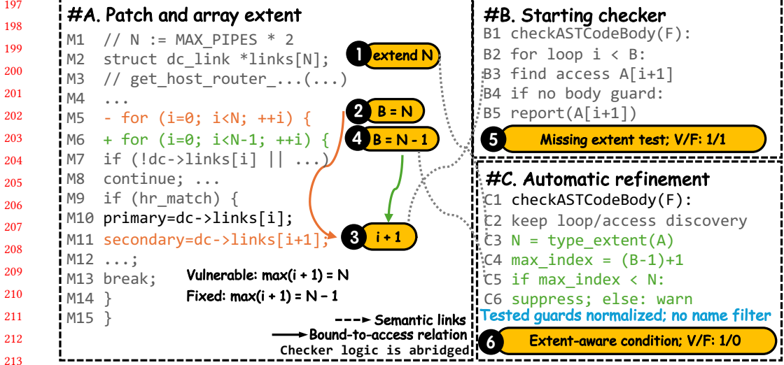
Fig. 1. Capacity-aware look-ahead refinement. Abridged code: N denotes \text{MAX\_PIPES} * 2 ; \text{hr\_match} denotes host-router equality. Original/refined vulnerable/fixed alerts are 1/1 and 1/0 in independent replay. The 14-response, model-produced illustration used fixture feedback and is separate from the one-response main-study checker. Orange/green solid arrows relate vulnerable/fixed bounds to the access; gray dotted links denote semantic correspondences. Code colors mark unsafe/patched bound and capacity logic.
