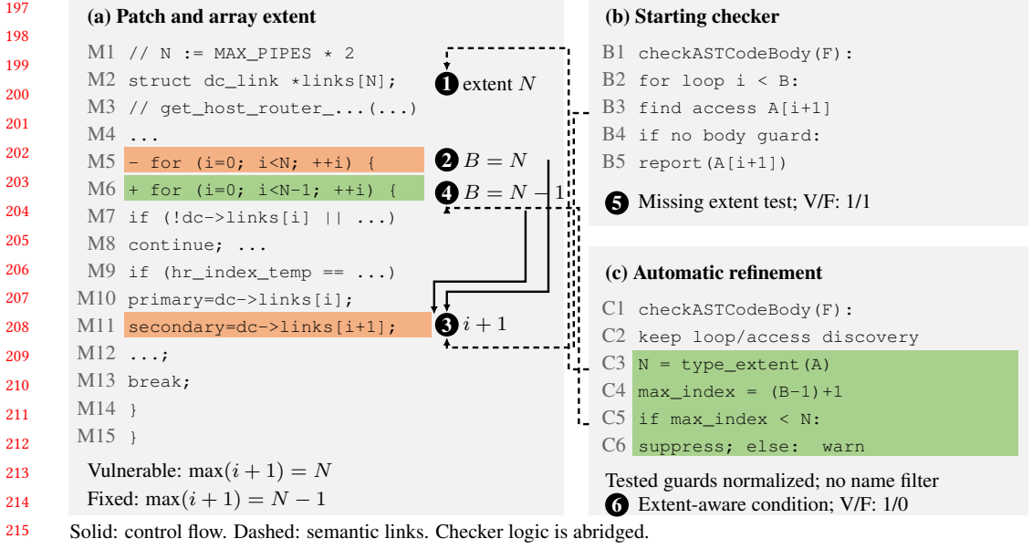
Fig. 1. Capacity-aware look-ahead refinement. Panel A combines an abridged array declaration and patch chunk; N denotes \text{MAX\_PIPES} * 2 . Panels B and C show abridged checker logic. The original checker reports 1/1 vulnerable/fixed alerts; the separately budgeted, 14-response model-produced illustration reports 1/0 in an independent execution replay. Its revisions used fixture feedback; it is not the one-response main-study checker. Solid arrows show control flow, dashed arrows semantic correspondences. Orange marks the unsafe bound/access and green the patched bound and capacity test.
