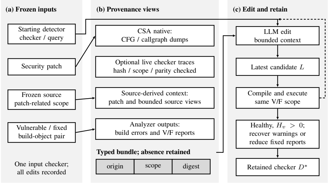
Fig. 2. SEMWEAVER architecture. A generated detector, patch and bounded evidence feed the editor and paired retention rule. Native provenance is checked separately from collector names. Retention tracks version-warning presence, not target correctness; fixed silence is secondary. Inputs, rejected/retained candidates and raw validation records remain auditable.
