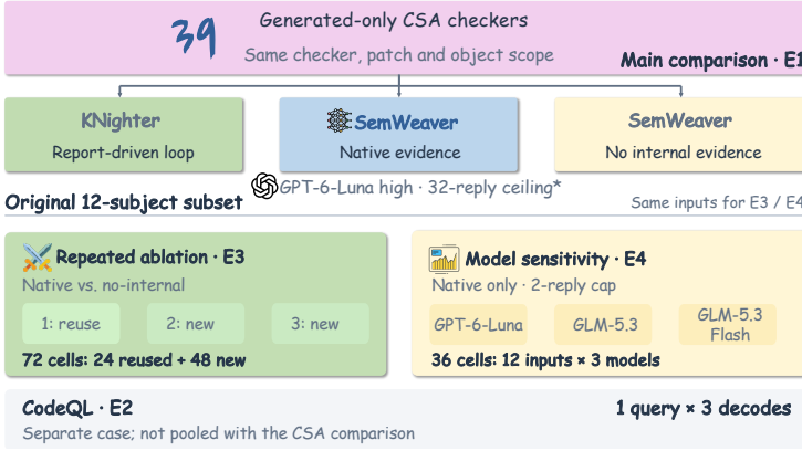
Fig. 3. Experimental design and reuse. E3’s first decode reuses E1; E4 uses the same 12 inputs, not another cohort. Cells are not independent bugs. *Audited natural-stop reuses retain original caps; shared ceilings do not imply equal realized effort.
