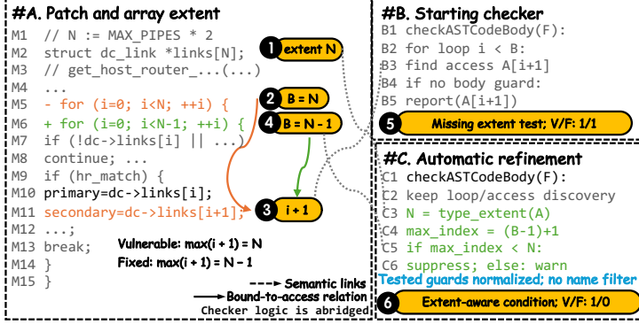
Fig. 1. Capacity-aware look-ahead refinement. Abridged code: N denotes \text{MAX\_PIPES} * 2 ; \text{hr\_match} denotes host-router equality. Original/refined vulnerable/fixed alerts are 1/1 and 1/0 in independent replay. The 14-response, model-produced illustration used fixture feedback and is separate from the one-response main-study checker. Orange/green solid arrows relate vulnerable/fixed bounds to the access; gray dotted links denote semantic correspondences. Code colors mark unsafe/patched bound and capacity logic.
