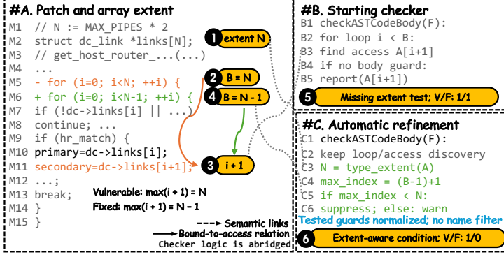
Fig. 1. Capacity-aware look-ahead refinement. Abridged code: N denotes \text{MAX\_PIPES} * 2 and \text{hr\_match} host-router equality. Independent vulnerable/fixed alerts change from 1/1 to 1/0. This 14-response illustration used fixture feedback and differs from the one-response main-study checker. Orange/green arrows connect the bounds to the access; gray dotted links mark semantic correspondences.
