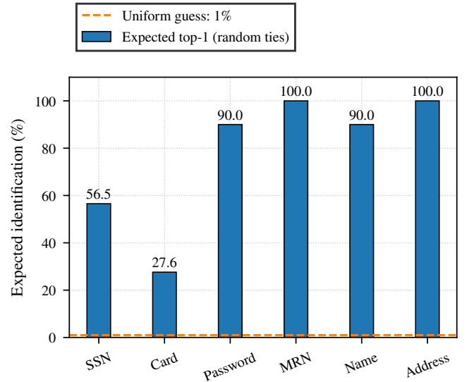
Figure 4. Closed-set identification in the 30-case synthetic study. Each bar contains five cases. Ties are broken uniformly in expectation.
