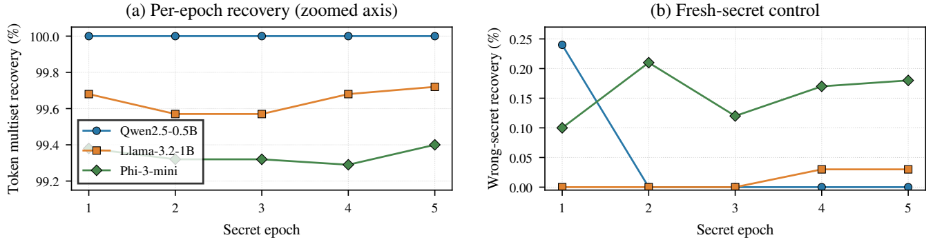
Figure 3. Secret-epoch stability on three models. Every epoch calibrates all heads. The y-axis in (a) is deliberately zoomed; (b) uses demixers from the wrong configuration. The conversations are not an exclusive held-out set.
