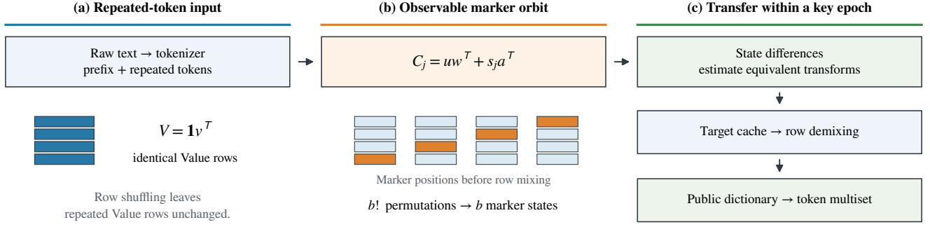
Figure 1. Attack mechanism. A legal repeat run makes first-layer Value rows identical. Fresh permutations move only the marker, producing a small orbit. The attacker recovers equivalent transforms from its own protected blocks, then matches demixed victim rows against a public-model dictionary. The diagram is schematic; no victim plaintext or server secret is an attack input.
