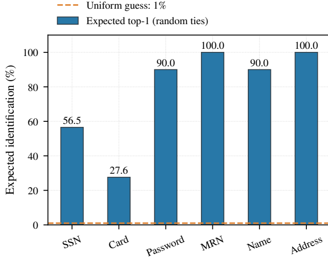
Figure 4. Closed-set identification in the 30-case synthetic study. Each bar contains five cases. Ties are broken uniformly in expectation.
