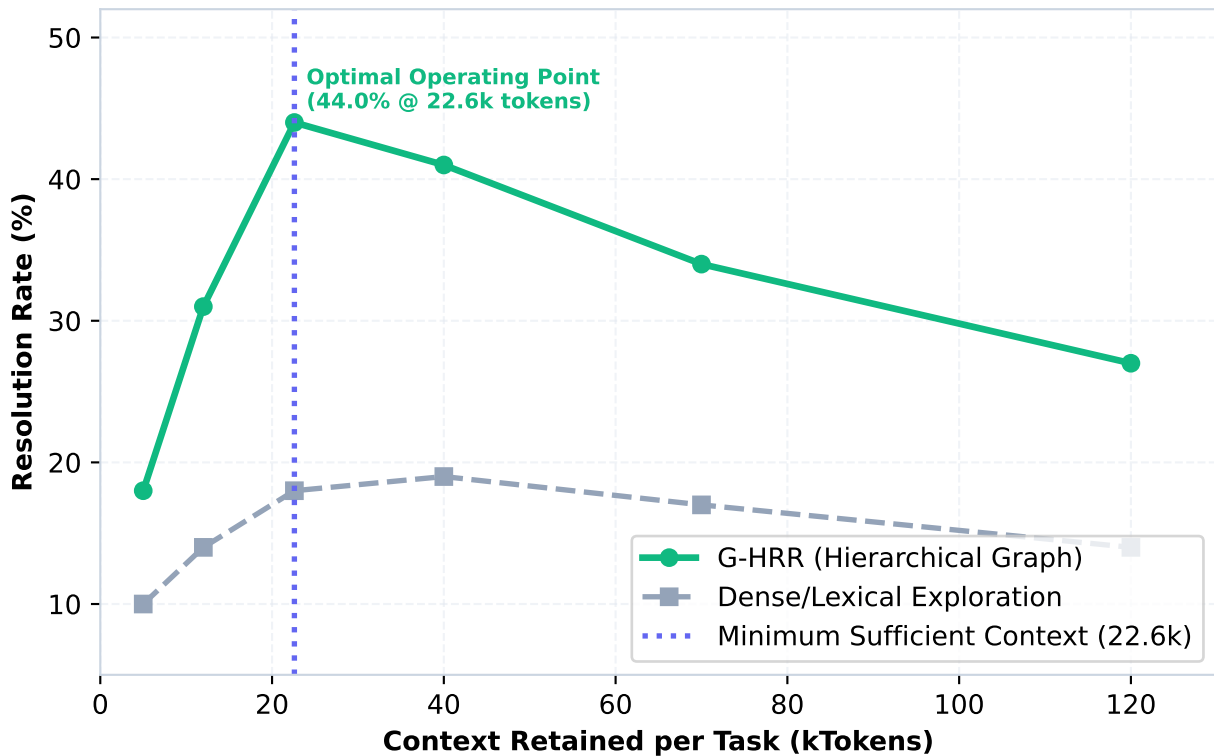
Figure 5: Resolution Rate vs. Context Budget (Context Sufficiency Frontier)
