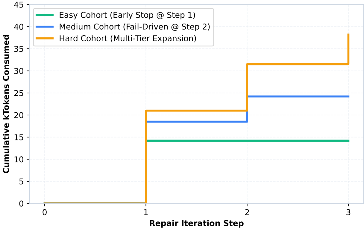
Figure 8: Adaptive Context Accumulation Trajectories Across Issue Complexities
