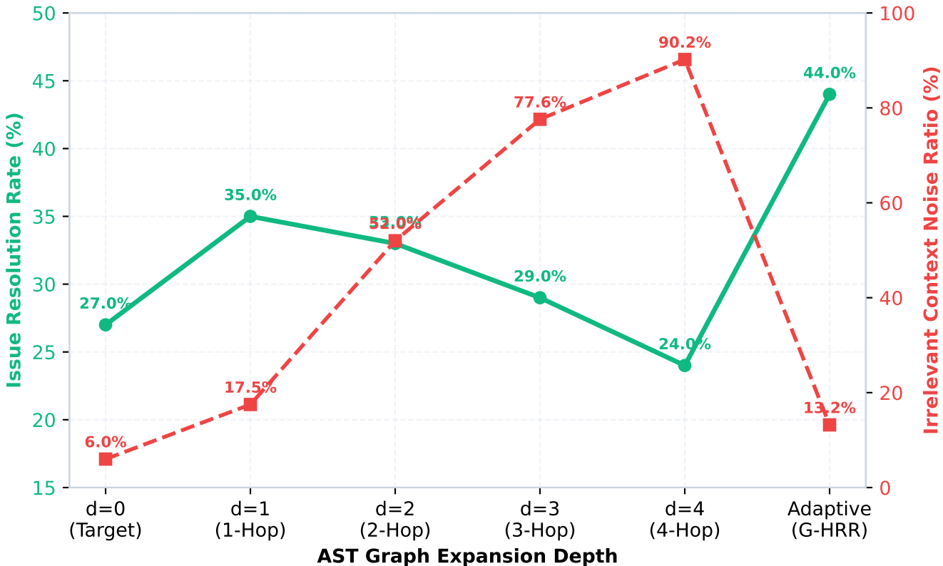
Figure 4: Non-Monotonicity of Graph Depth vs. Context Dilution Noise
