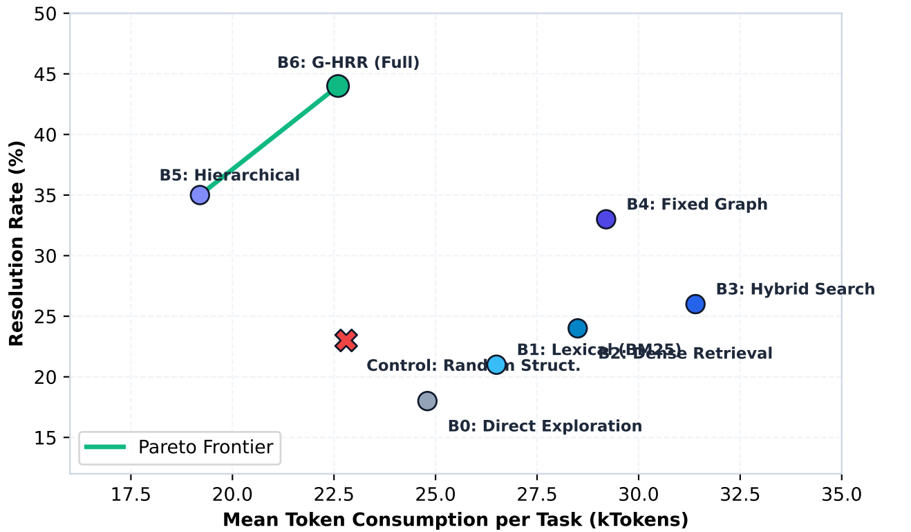
Figure 6: Performance-Efficiency Frontier (Including Red-Team Random Control)
