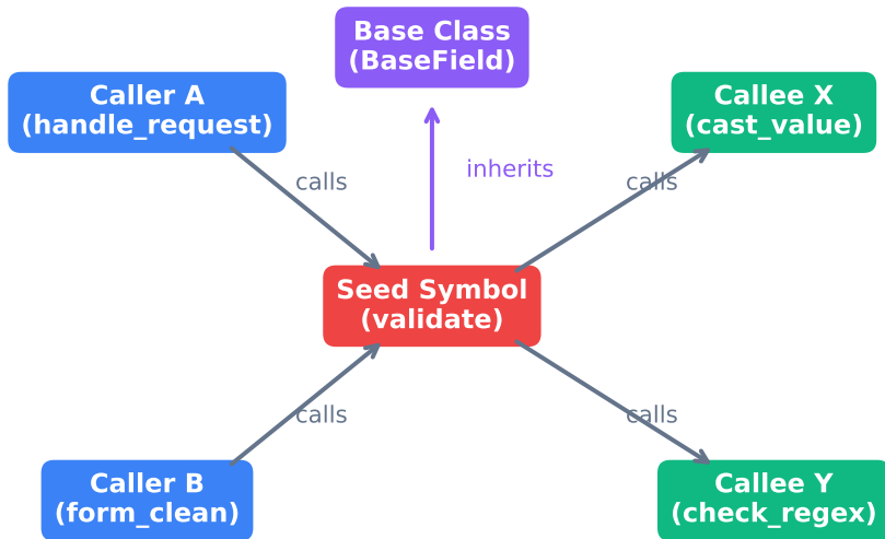
Figure 2: 1-Hop AST Dependency Subgraph Topology
