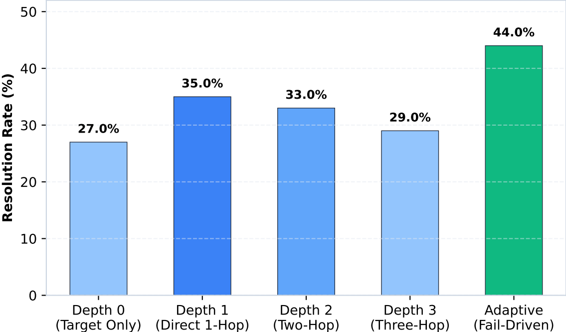
Figure 3: SWE-bench Resolution Rate vs. Graph Expansion Depth (H6 Validation)
