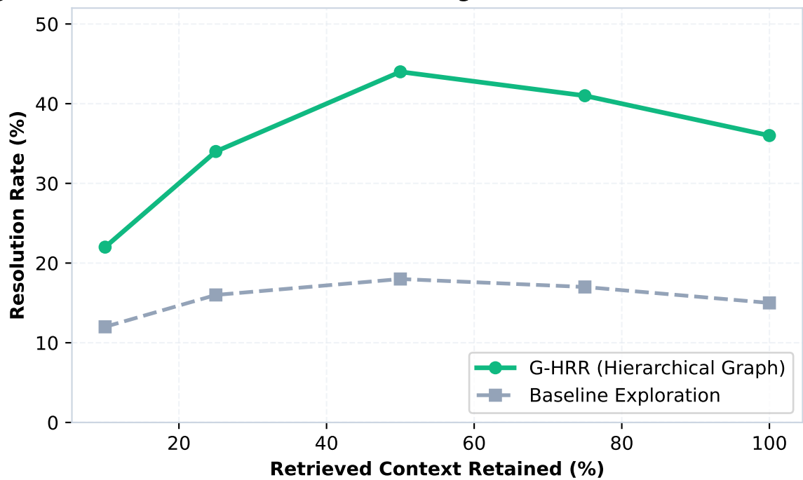
Figure 4: Resolution Rate vs. Context Budget (Context Pollution Demonstration)
