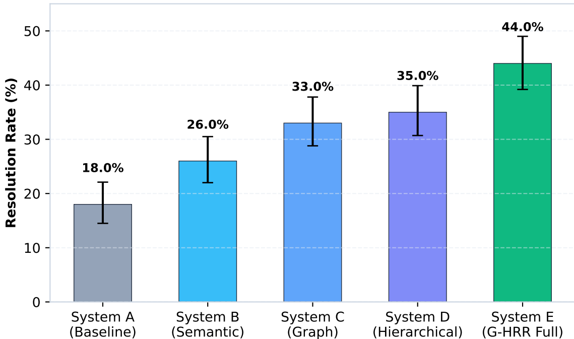
Figure 5: Comparative Issue Resolution Rate on SWE-bench Cohort
