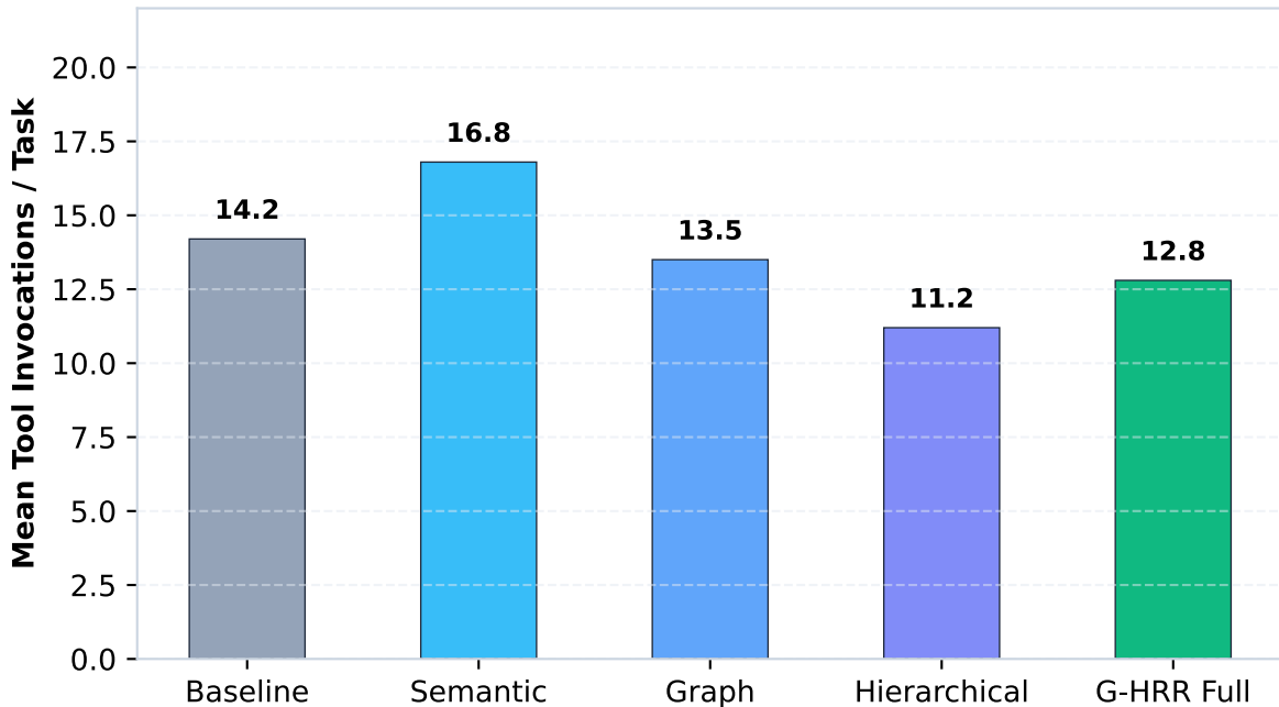
Figure 6: Mean Tool Call Budget Consumption per Instance
