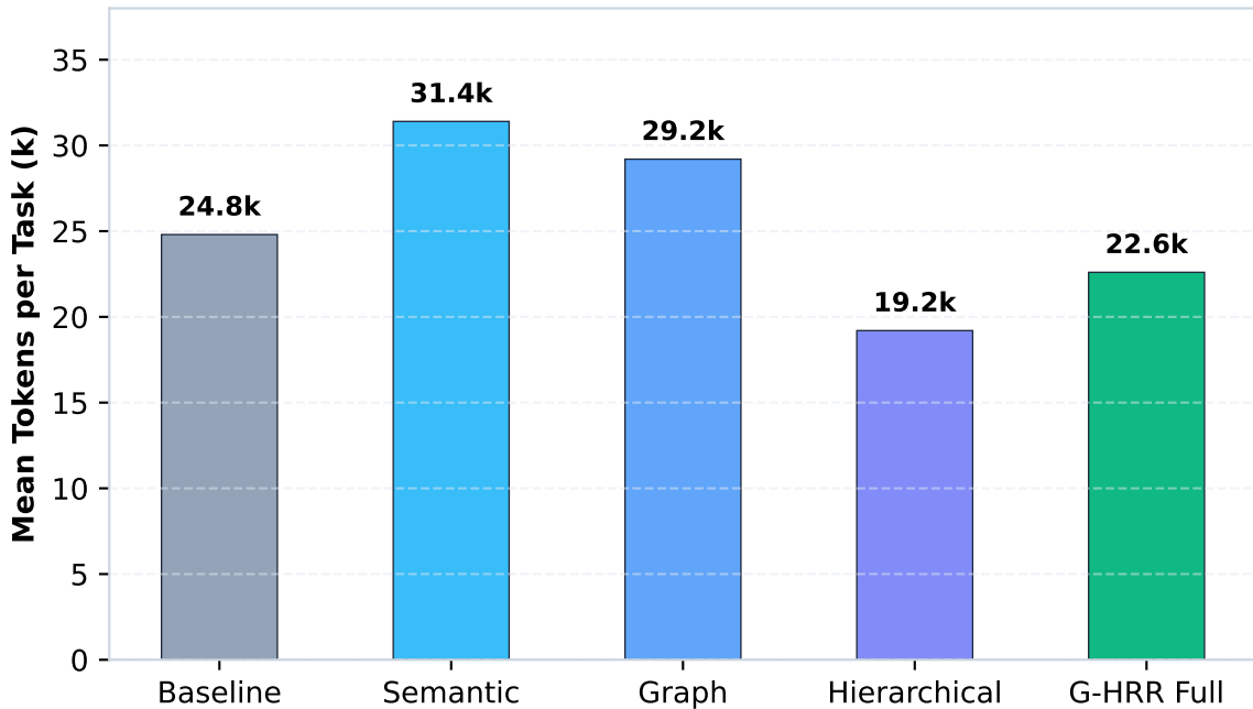
Figure 7: Mean Prompt and Generation Token Consumption (kTokens)
