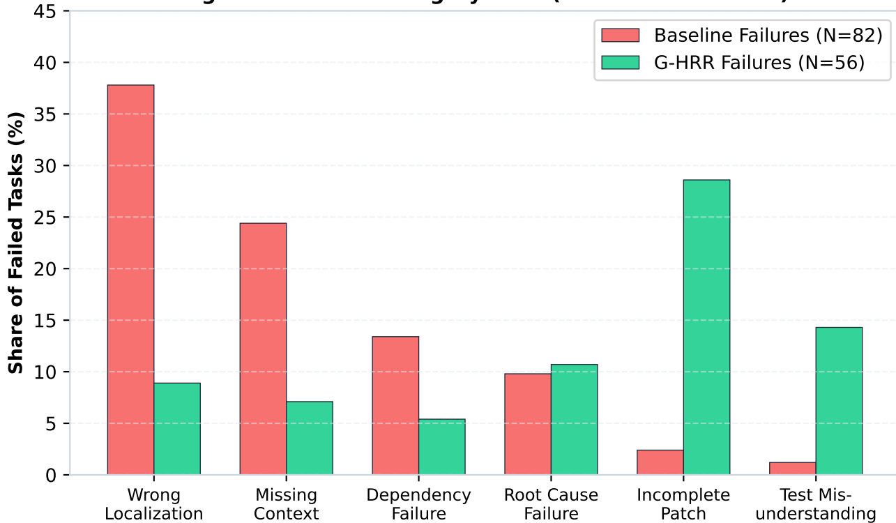
Figure 8: Failure Category Shift (Baseline vs. G-HRR)
