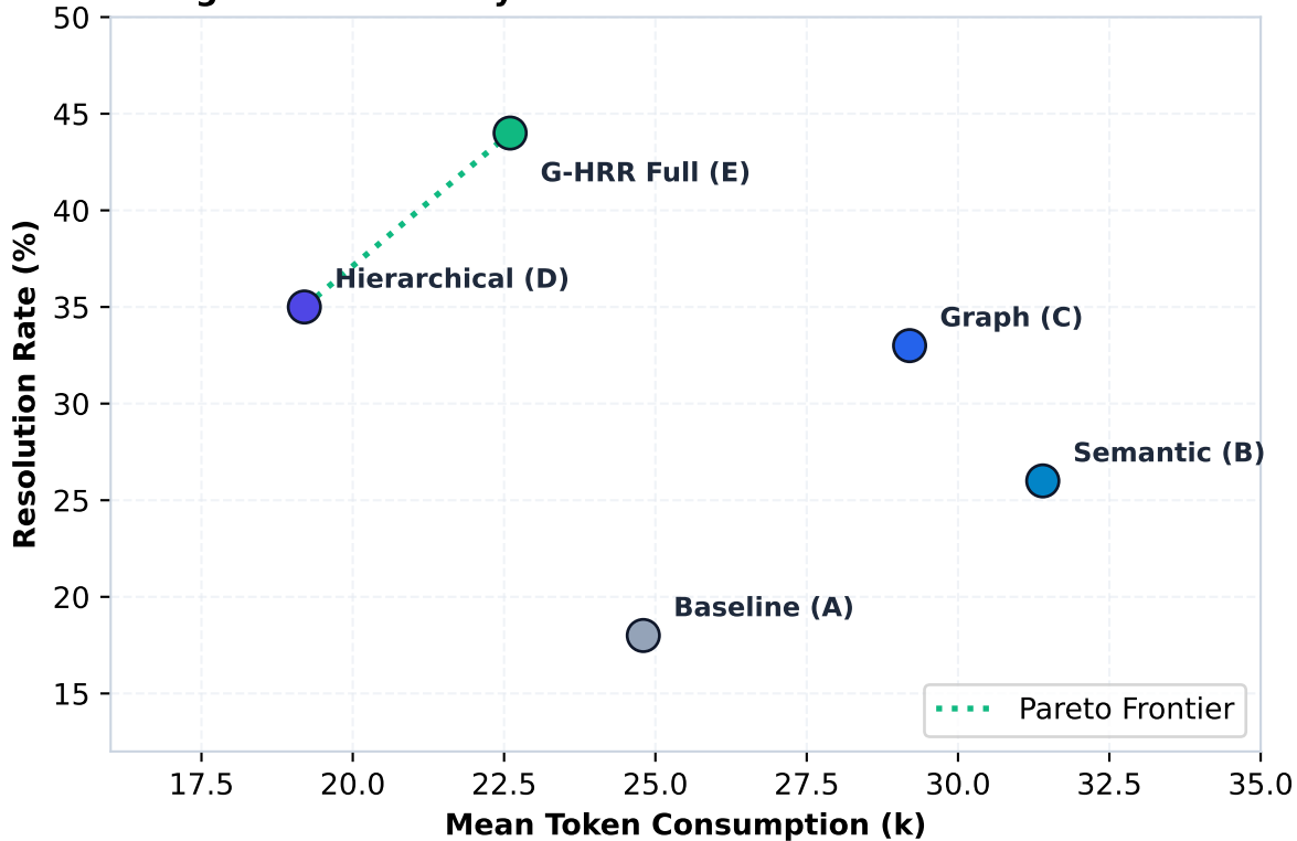
Figure 9: Efficiency Frontier: Success Rate vs. Token Cost
