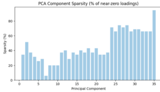
Figure 7.1.2: Sparsity Pattern of all Principal Components (percentage of loadings near zero)
