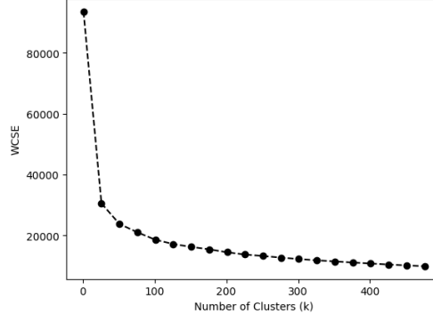
Figure 7.3.1.1: Number of Clusters vs. Weighted Sum of Square Errors. Throughout the training of the KDS, we set the hidden size k = 90 .
