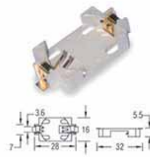
CH28-2032 FOR CR2032
