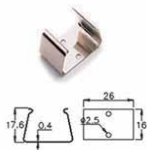
BH980-1 HOLDER
