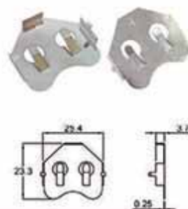
BH980 HOLDER
