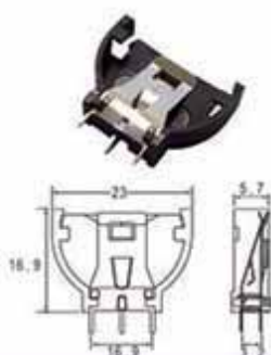
CH261-2032 FOR CR2032
