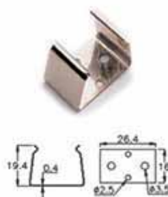
BH980-2 HOLDER
