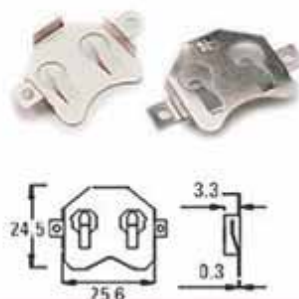
BC-2404 FOR CR2450
