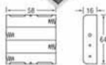
BH342-1A BH342-1B BH342-1D FOR FOUR "AA" CELLS
