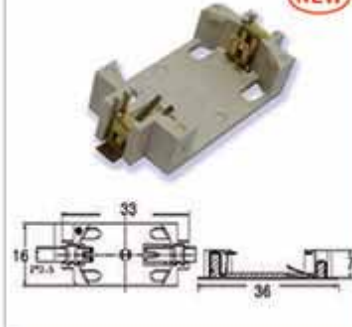
CH274-2450 FOR CR2450
