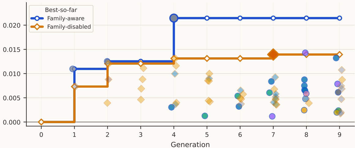
Discovery score
