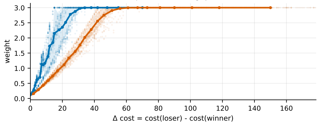
JSSP over cost gap
