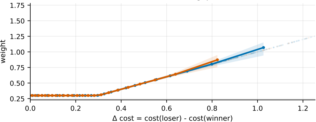
FFSP over cost gap
