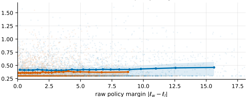
FFSP over raw policy margin
