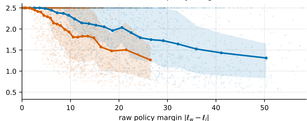
JSSP over raw policy margin
