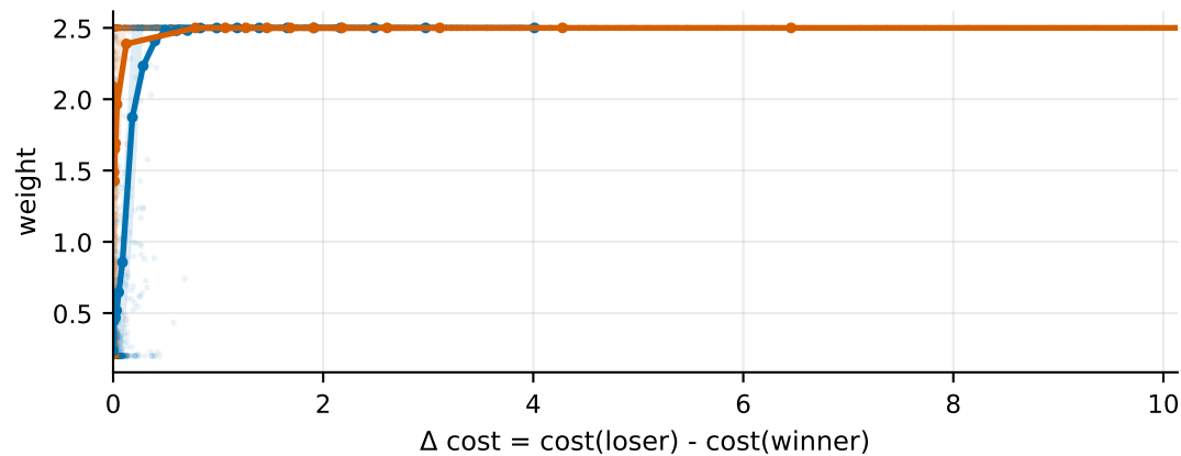
CVRP over cost gap
