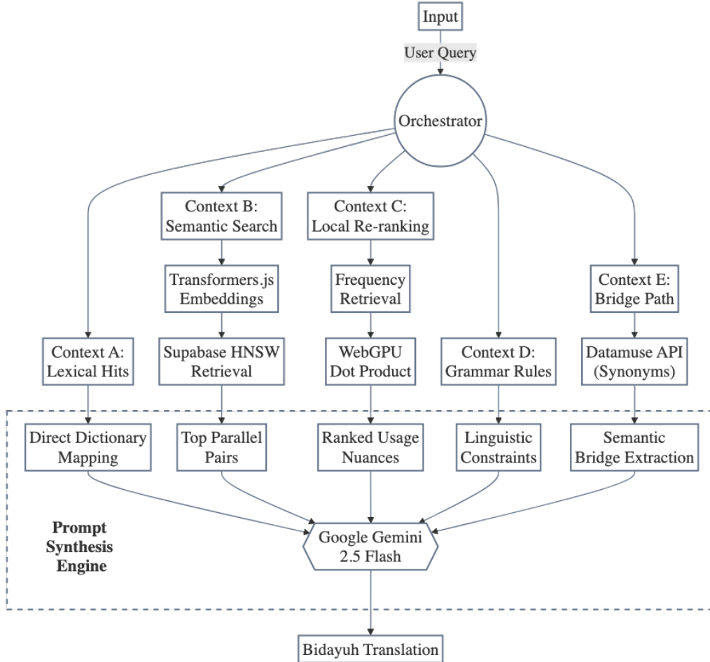
Figure 2. The 5-Stage Context Assembly Pipeline.
