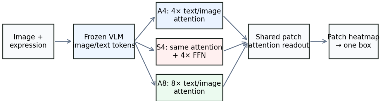
Figure 1. The frozen VLM stays unchanged. The only causal intervention is the trainable decoder's FFN residual; A8 tests capacity reallocation rather than a compute-matched alternative.
