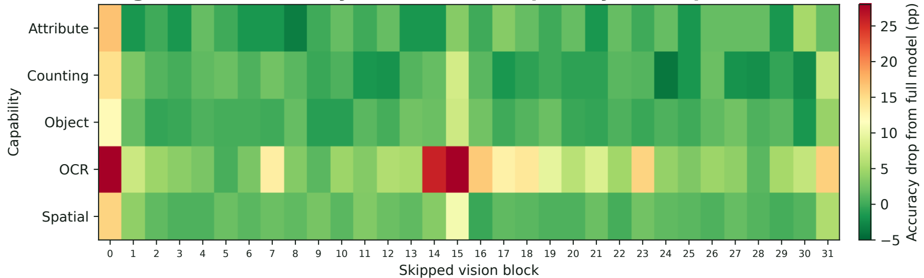
Single-block sensitivity varies across capability and depth
