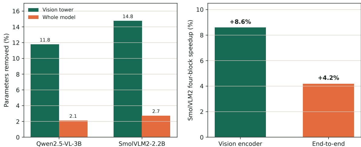
Figure 8: Four-block parameter fractions for both models and measured SmolVLM2 latency. The latency measurement is an unlocked same-VM comparison on one RTX 4090, not fixed-clock or edge-device evidence.
