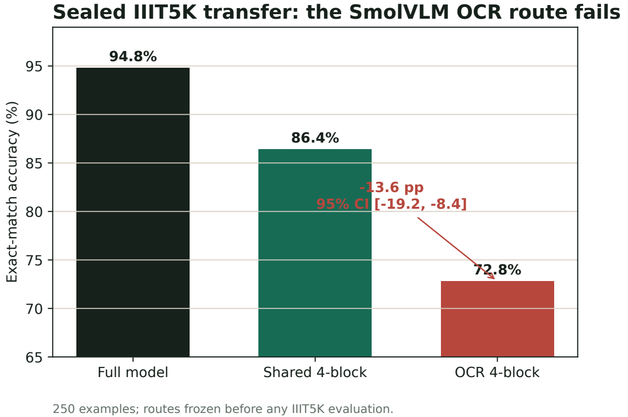
Figure 6: Post-freeze source transfer on IIIT5K. Both compressed conditions skip four SmolVLM2 vision blocks. Routes and all evaluation choices were frozen before any IIIT5K prediction was produced.
