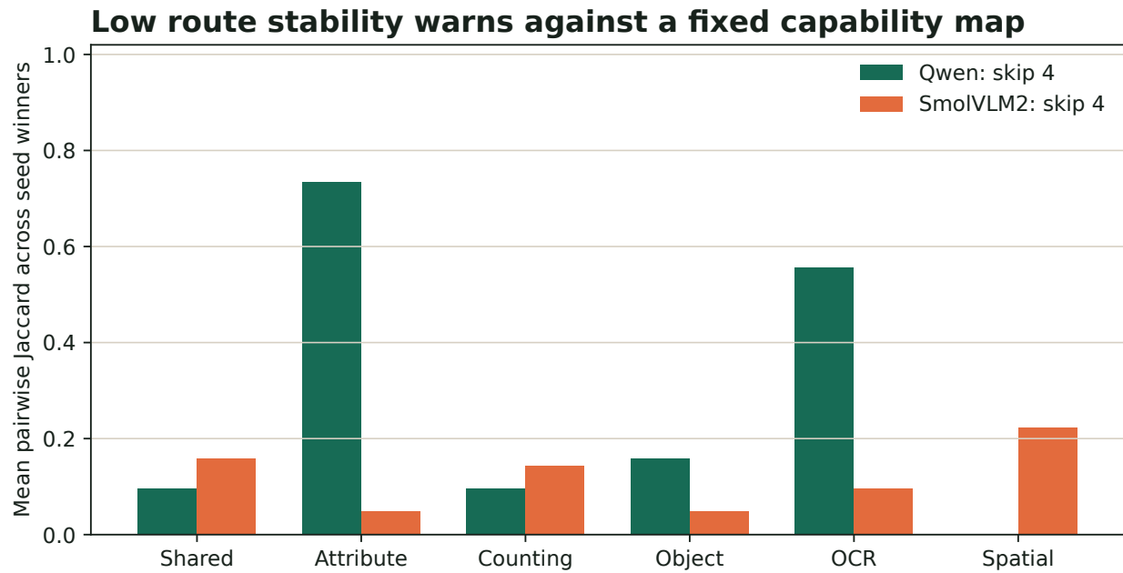
Figure 7: Mean pairwise Jaccard overlap among three seed-level four-block development winners. Low overlap indicates that the frozen route is one strong solution among several distinct candidates, not a uniquely identified block map.
